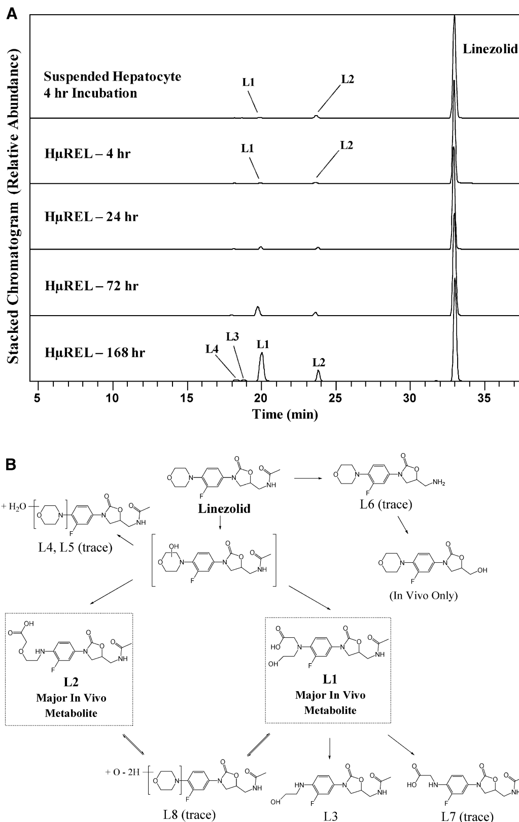
Fig. 3. (A) Extracted ion chromatograms showing the metabolite profile of linezolid following incubations in human suspended hepatocytes (4 hours) and the HμREL model (up to 7 days). (B) Proposed metabolic pathways of linezolid. Metabolites highlighted in boxes are consistent with previously published human metabolite data. In vivo data were obtained from Slatter et al. (2001).
