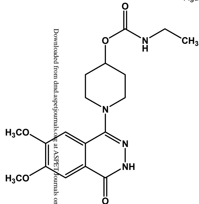
4-Oxo-Carbazeran
