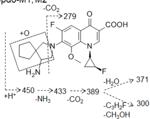
Cpd6-M4
