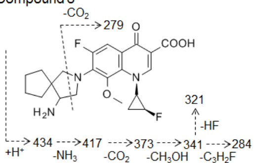
Compound 6
