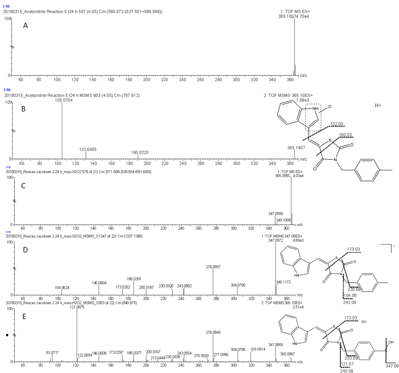
Supplementary Figure 1. Spectra of M1 and M2 from microsome incubation experiments and from biomimetic oxidation system. (A) Spectrum of the [M+H]^+ of the putative structure M1. (B) MS^2 signals of the selected ion 365 at retention time of M1 and the proposed fragmentation sites. (C) Spectrum showing the [M+H]^+ and the in source fragment [M+H-H_2O]^+ of the \alpha -hydroxylated metabolite M2. (D) MS^2 signals of the selected ion 347 at the retention time of M2 and the proposed fragmentation sites. (E) MS^2 signals of the selected ion 365 at the retention time of M2 and the proposed fragmentation sites.
