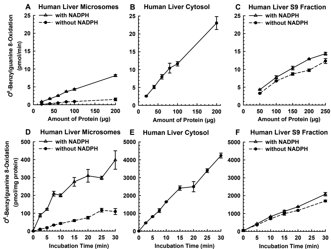
Supplemental Fig. S3. O 6 -Benzylguanine 8-oxidation catalyzed by human liver microsomes, cytosol, and S9 fraction as a function of amount of protein and incubation time. (A) Microsomes (20, 40, 60, 80, 100, or 200 μg protein) was incubated with O 6 -benzylguanine (10 μM) in the absence and presence of NADPH (1 mM) at 37°C for 10 min. (B) Cytosol (20, 40, 60, 80, 100, or 200 μg protein) was incubated with O 6 -benzylguanine (10 μM) at 37°C for 10 min. (C) S9 fraction (50, 100, 150, 200, or 250 μg protein) was incubated with O 6 -benzylguanine (10 μM) in the absence and presence of NADPH (1 mM) at 37°C for 10 min. (D) Microsomes (60 μg protein) was incubated with O 6 -benzylguanine (10 μM) in the absence and presence of NADPH (1 mM) at 37°C for 0, 2.5, 5, 7.5, 10, 15, 20, 25, or 30 min. (E) Cytosol (20 μg protein) was incubated with O 6 -benzylguanine (10 μM) at 37°C for 0, 2.5, 5, 7.5, 10, 15, 20, 25, or 30 min. (F) S9 fraction (60 μg protein) was incubated with O 6 -benzylguanine (10 μM) in the absence and presence of NADPH (1 mM) at 37°C for 0, 5, 10, 15, 20, or 30 min. Data are expressed as mean ± S.E.M. of three independent experiments conducted in duplicate or triplicate.
