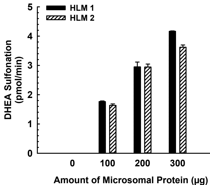
Supplemental Fig. S5. DHEA sulfonation in enzymatic incubations containing cytosol-contaminated human liver microsomes. DHEA (1 µM) was incubated with microsomes (0, 100, 200, or 300 µg protein; Pool 1 and Pool 2) and 3'-phosphoadenosine 5'-phosphosulfate (5 µM) at 37°C for 30 min. Data are expressed as mean ± S.E.M. of three independent experiments.
