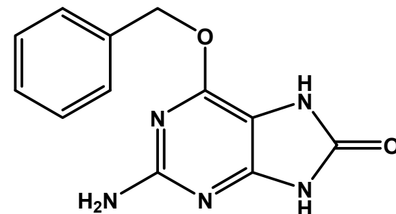
8-Oxo-O 6 -Benzylguanine
