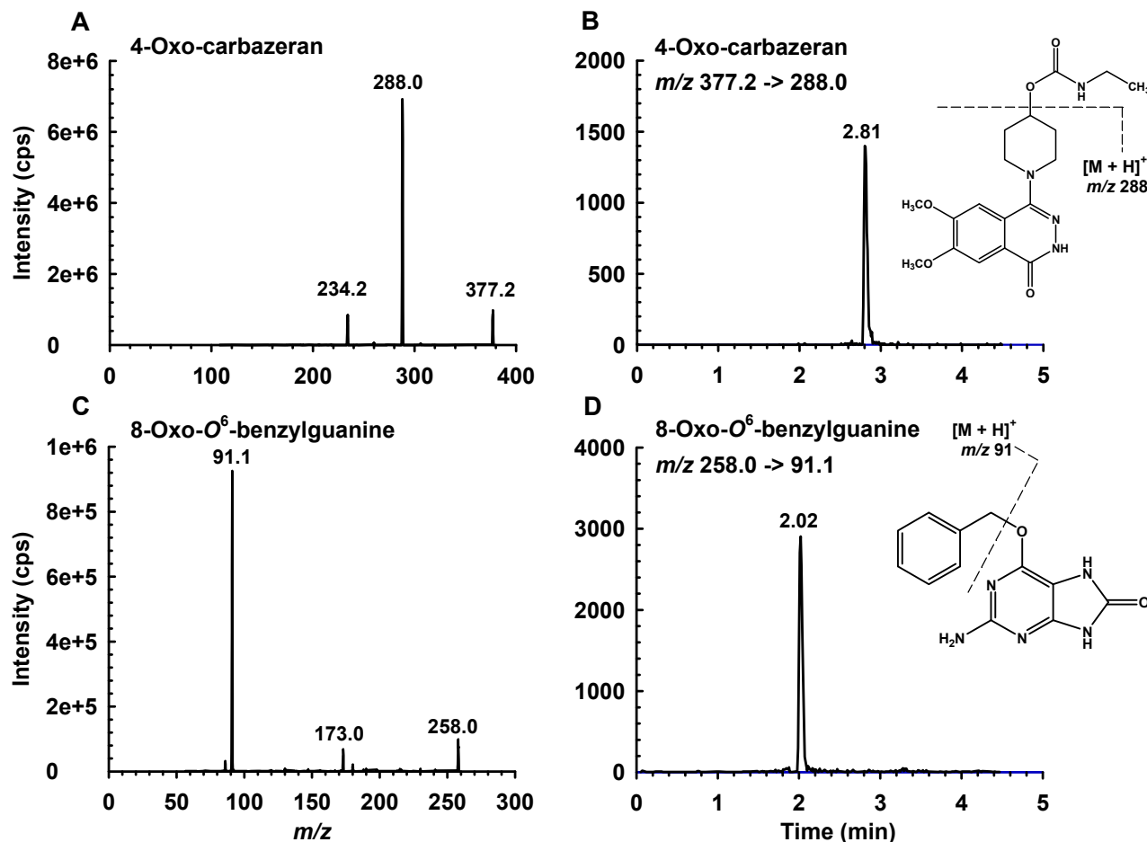
Supplemental Fig. S1. Representative product ion mass spectra and chromatograms of 4-oxo-carbazeran and 8-oxo- O 6 -benzylguanine. (A, C) A solution of 1 \mu\text{g/ml} of 4-oxo-carbazeran (A) or 8-oxo- O 6 -benzylguanine (C) in 50% acetonitrile containing 0.1% formic acid was infused directly into the mass spectrometer, and the product ion mass spectra of each analyte are shown. (B, D) Calibration standard samples containing potassium phosphate buffer (100 mM; pH 7.4), substrate (0.5 \mu\text{M} of carbazeran or 5 \mu\text{M} of O 6 -benzylguanine), standard analyte (2 pmol of 4-oxo-carbazeran or 8-oxo- O 6 -benzylguanine), and internal standard (25 nM of tolbutamide) were analyzed by UPLC-MS/MS in the multiple reaction monitoring mode. Shown are the chromatograms for 4-oxo-carbazeran (B) and 8-oxo- O 6 -benzylguanine (D), as determined with a m/z transition of 377.2 \rightarrow 288.0 and 258.0 \rightarrow 91.1, respectively.
