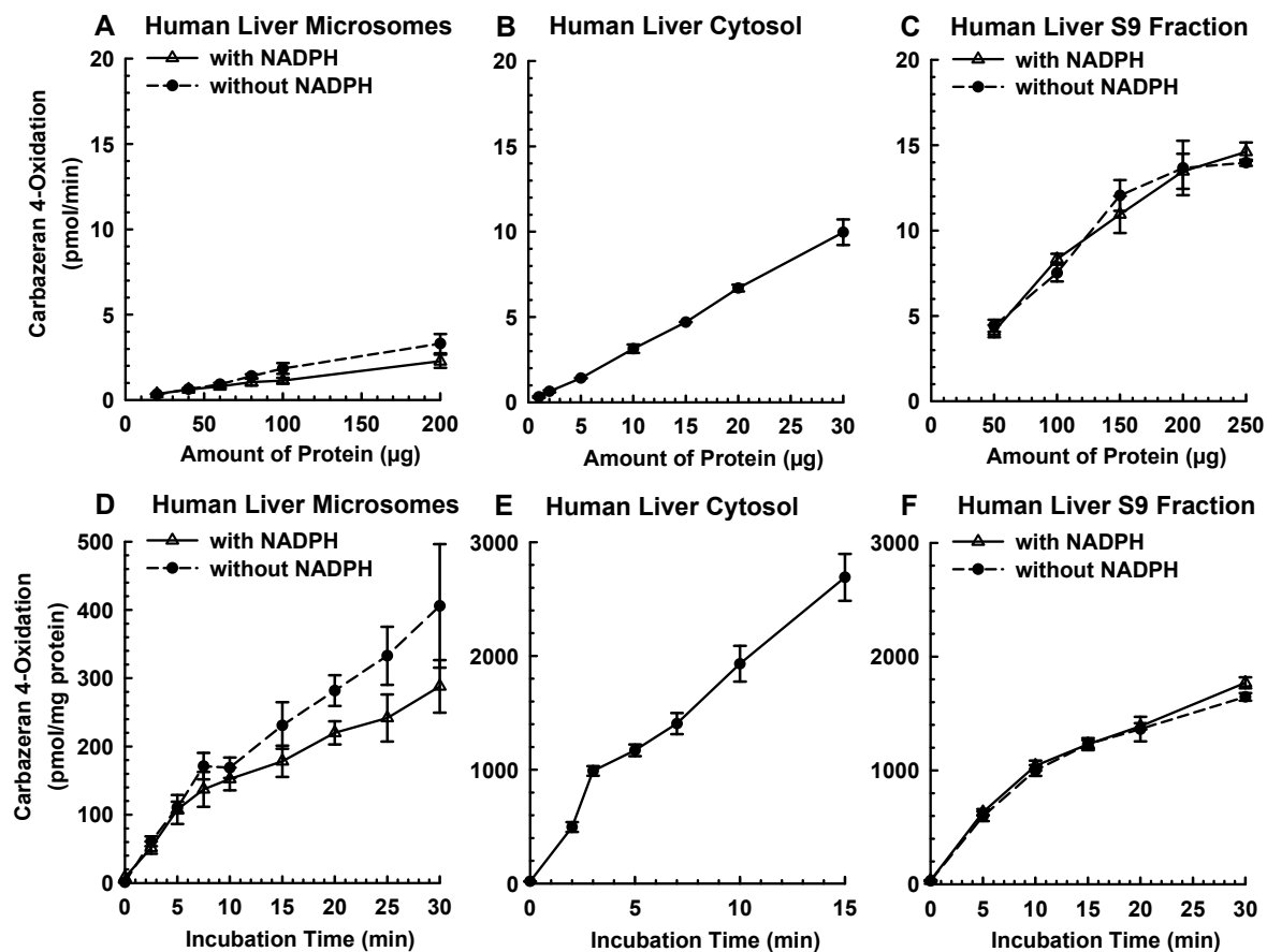
Supplemental Fig. S2. Carbazeran 4-oxidation catalyzed by human liver microsomes, cytosol, and S9 fraction as a function of amount of protein and incubation time. (A) Microsomes (20, 40, 60, 80, 100, or 200 µg protein) was incubated with carbazeran (1 µM) in the absence and presence of NADPH (1 mM) at 37°C for 5 min. (B) Cytosol (1, 2, 5, 10, 15, 20, or 30 µg protein) was incubated with carbazeran (1 µM) at 37°C for 3 min. (C) S9 fraction (50, 100, 150, 200, or 250 µg protein) was incubated with carbazeran (1 µM) in the absence and presence of NADPH (1 mM) at 37°C for 5 min. (D) Microsomes (100 µg protein) was incubated with carbazeran (1 µM) in the absence and presence of NADPH (1 mM) at 37°C for 0, 2.5, 5, 7.5, 10, 15, 20, 25, or 30 min. (E) Cytosol (20 µg protein) was incubated with carbazeran (1 µM) at 37°C for either 0, 2, 3, 5, 7, 10, or 15 min. (F) S9 fraction (60 µg protein) was incubated with carbazeran (1 µM) in the absence and presence of NADPH (1 mM) at 37°C for 0, 5, 10, 15, 20, or 30 min. Data are expressed as mean ± S.E.M. of three independent experiments conducted in duplicate or triplicate.
