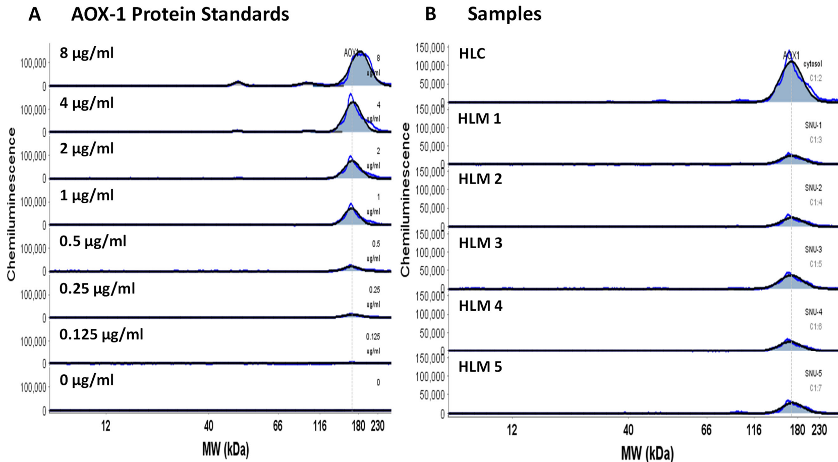
Supplemental Fig. S4. AOX-1 protein expression in human liver cytosol and various pools of human liver microsomes. AOX-1 protein levels were quantified by a capillary nano-proteomic immunoassay. Shown are representative plots of chemiluminescent signal versus molecular weight for AOX-1 protein standards (0.125-8 µg/ml) (A), human liver cytosol (HLC) (B), and five pools of human liver microsomes (HLM 1 to HLM 5) (B). The peak area was used to plot the calibration curve and calculate the concentration of AOX-1 protein in each sample. Data shown are a representative of three independent experiments.
