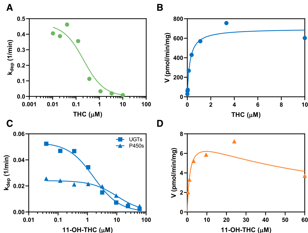
Fig. 1. Representative kinetic profiles of (A) THC depletion, (B) 11-OH-THC formation, (C) 11-OH-THC depletion by UGT and P450 enzymes, and (D) COOH-THC formation in pooled HLMs from one (of three to four) independent experiment, each with duplicate determinations. Depletion rate constant ( k_{\text{dep}} ) and formation rate ( V ) were obtained from cannabinoid concentration–time profiles (see Supplemental Fig. 1 for representative profiles). Substrate depletion (eq. 5) and metabolite formation (eq. 7) were used to determine kinetic parameters ( V_{\text{max}} and K_{\text{m}} ). A substrate inhibition model (eq. 8) was used to model COOH-THC formation kinetics. Kinetic parameters estimated from these data were used as initial estimates for the subsequent modeling of cannabinoid depletion and formation kinetics using the P450 and UGT kinetics models shown in Fig. 3.
