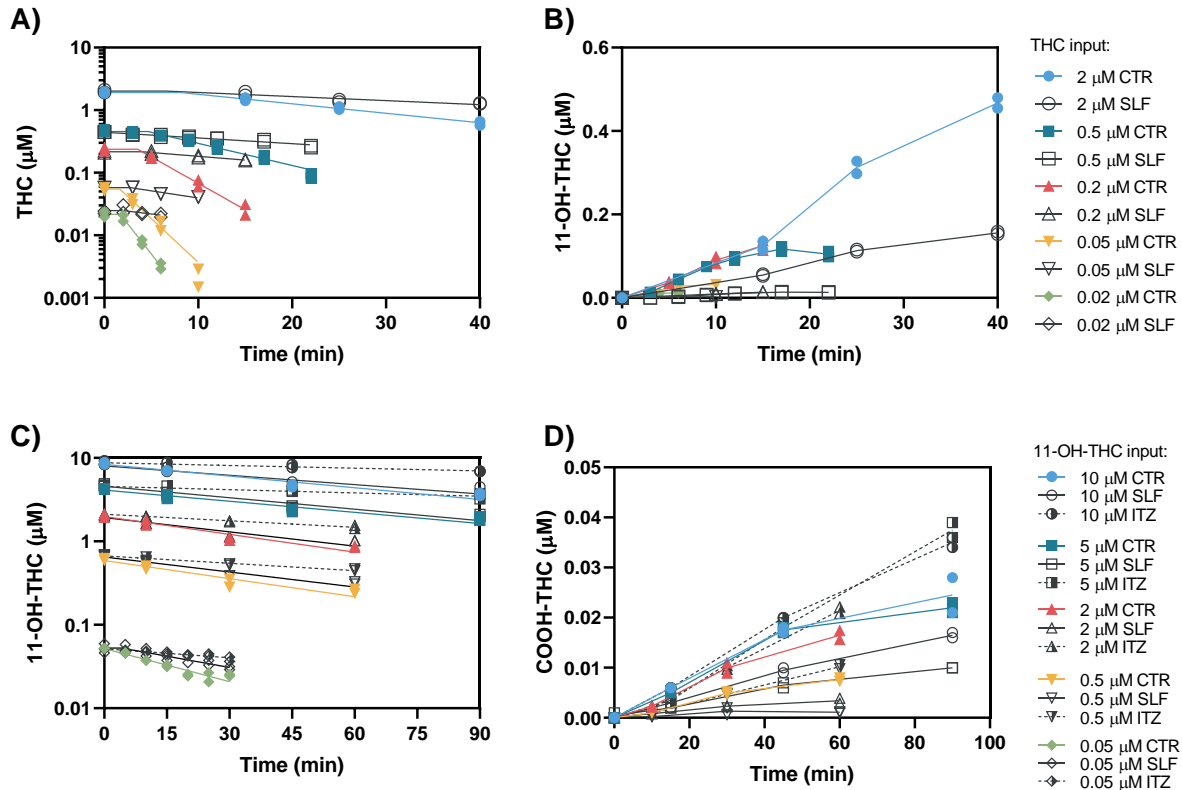
Supplementary Figure 2. Representative concentration-time profiles of A) THC depletion and B) 11-OH-THC formation at different THC concentrations in the absence (control, CTR) and presence of sulfaphenazole (SLF; CYP2C9 inhibitor) in pooled HLMs. Representative concentration-time profiles of C) 11-OH-THC depletion by P450 enzymes D) COOH-THC formation at different 11-OH-THC concentrations in the absence and presence of SLF and itraconazole (ITZ; CYP3A inhibitor) pooled HLMs. These experiments were conducted with limited THC/11-OH-THC concentrations that are within the nonlinear range (see Fig. 1 ). k_{\text{dep}} and V were obtained as described in Supplementary Fig. 1 . Data shown is representative from one (of three) independent experiments, each with duplicate determinations.
