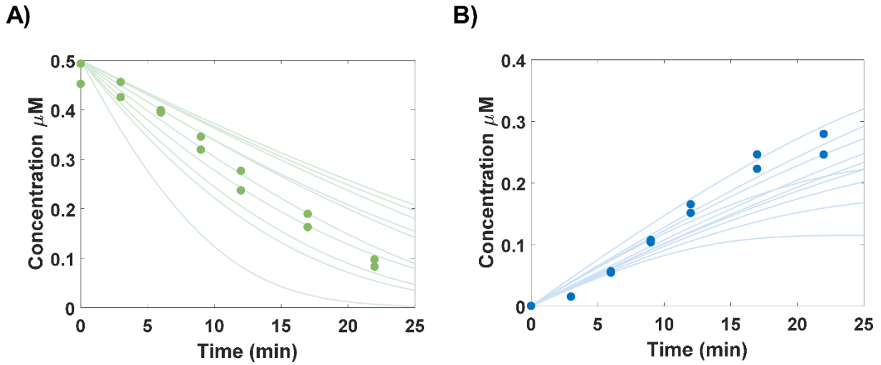
Supplementary Figure 4. Monte-Carlo simulations (lines, 10 individual simulations) using P450 kinetic model estimates ( Table 3 ) shows good agreement with observed concentrations (dots) from an independent dataset with duplicate determinations of A) 500 nM THC depletion and subsequent B) 11-OH-THC formation in pooled HLMs.
