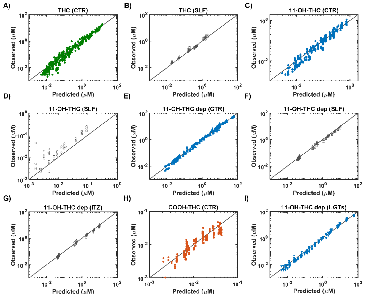
Supplementary Figure 3. Predicted versus observed concentrations (dots) and the line of unity for P450 (panels A-H) and UGT (panel I) kinetic models.
