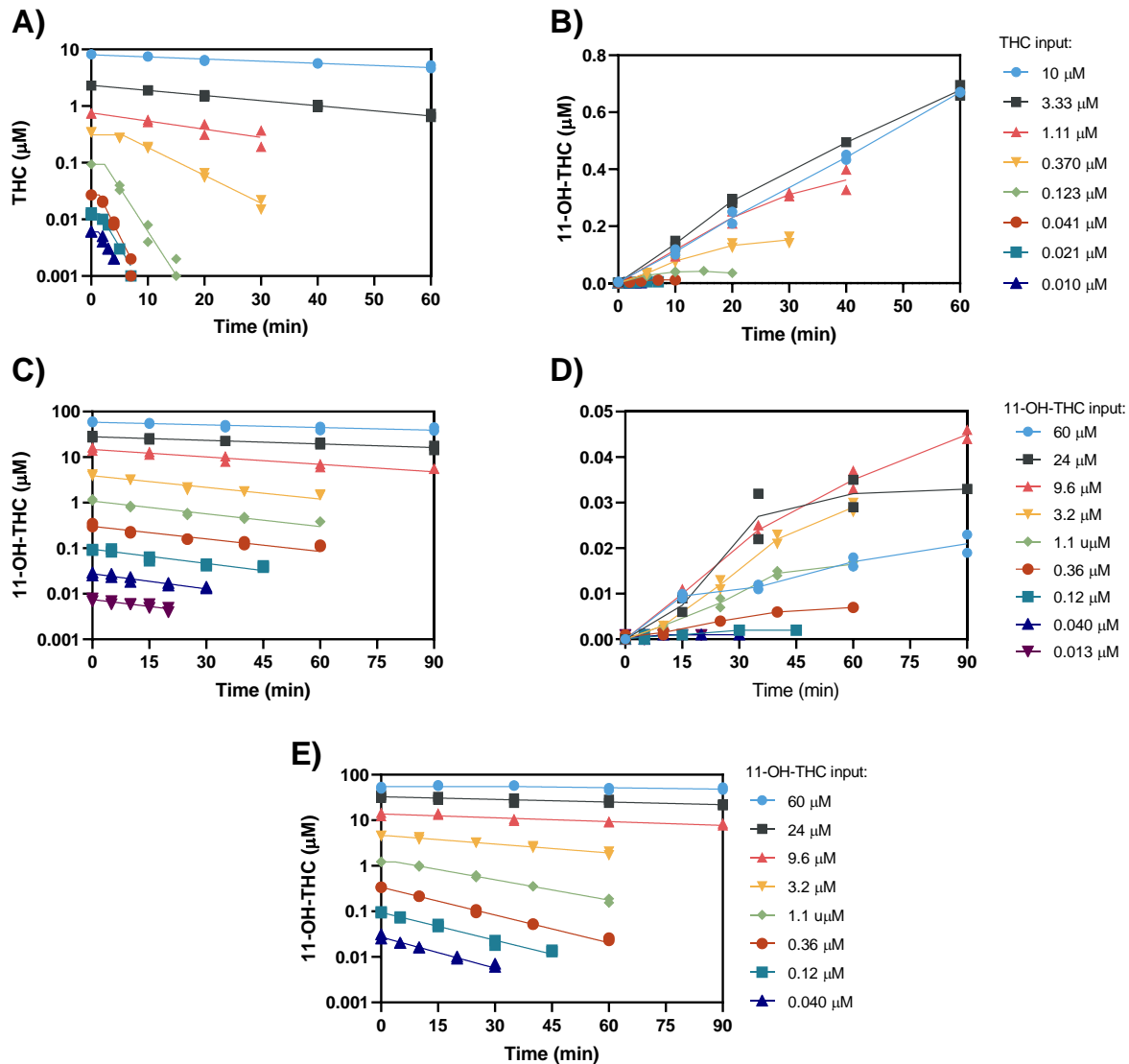
Supplementary Figure 1. Representative concentration-time profiles of A) THC depletion and B) 11-OH-THC formation at different THC concentrations in pooled HLMs. Representative concentration-time profiles of C) 11-OH-THC depletion by P450 enzymes D) COOH-THC formation and E) 11-OH-THC depletion by UGT enzymes at different 11-OH-THC concentrations in pooled HLMs. Depletion rate constant ( k_{\text{dep}} ) was obtained by fitting Eq. 5 to the concentration-time curves (panels A, C, E). Formation rate ( V ) was obtained through linear fit of the metabolite concentration-time profile of timepoints that corresponded to <20% parent
