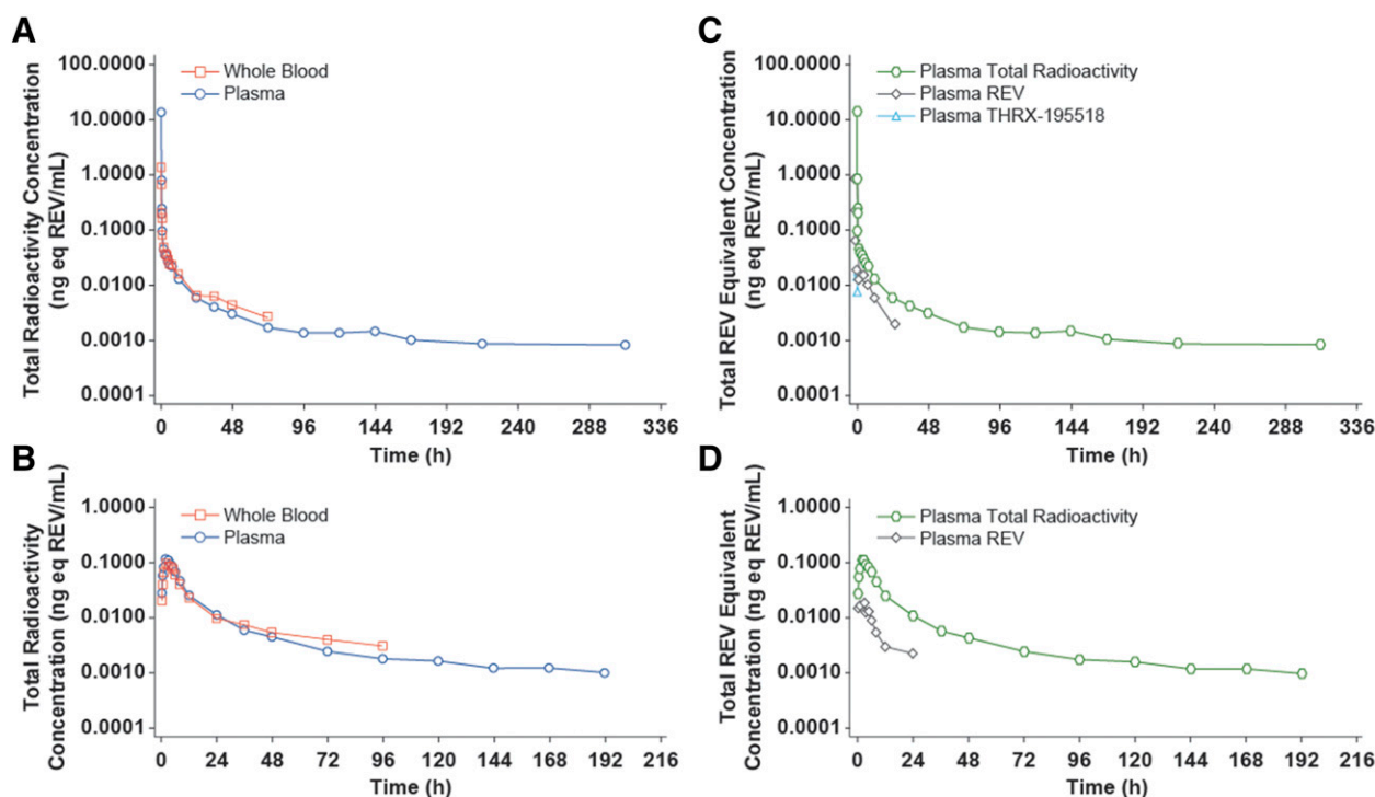
Fig. 2. Total radioactivity in whole blood and plasma over time (A) after a single intravenous dose of 20 \mu\text{g} [ ^{14}\text{C} ]-revefenacin ( n = 6 ) and (B) after a single oral dose of 200 \mu\text{g} [ ^{14}\text{C} ]-revefenacin ( n = 6 ). Total radioactivity, revefenacin, and THRX-195518 concentrations in plasma over time (C) after a single intravenous dose of 20 \mu\text{g} [ ^{14}\text{C} ]-revefenacin ( n = 6 ) and (D) after a single oral dose of 200 \mu\text{g} [ ^{14}\text{C} ]-revefenacin ( n = 6 ) and arithmetic mean. h, hour; REV, revefenacin.
