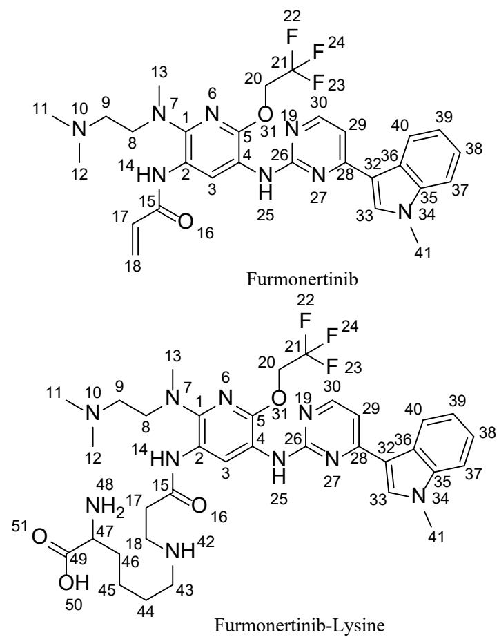
Supp. Fig.1 The structures of 1H and 13C of furmonertinib and furmonertinib-lysine
