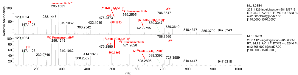
Fig. 5. Structural identification of furmonertinib-ASSAKQR adducts (A) and furmonertinib-LKASLQK adducts from human plasma incubated with the drug ex vivo (B).
