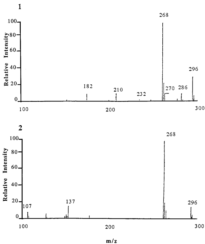
FIG. 6. CI-Mass spectrum of fungal metabolite C: 1) Metabolite C; 2) P9400.
