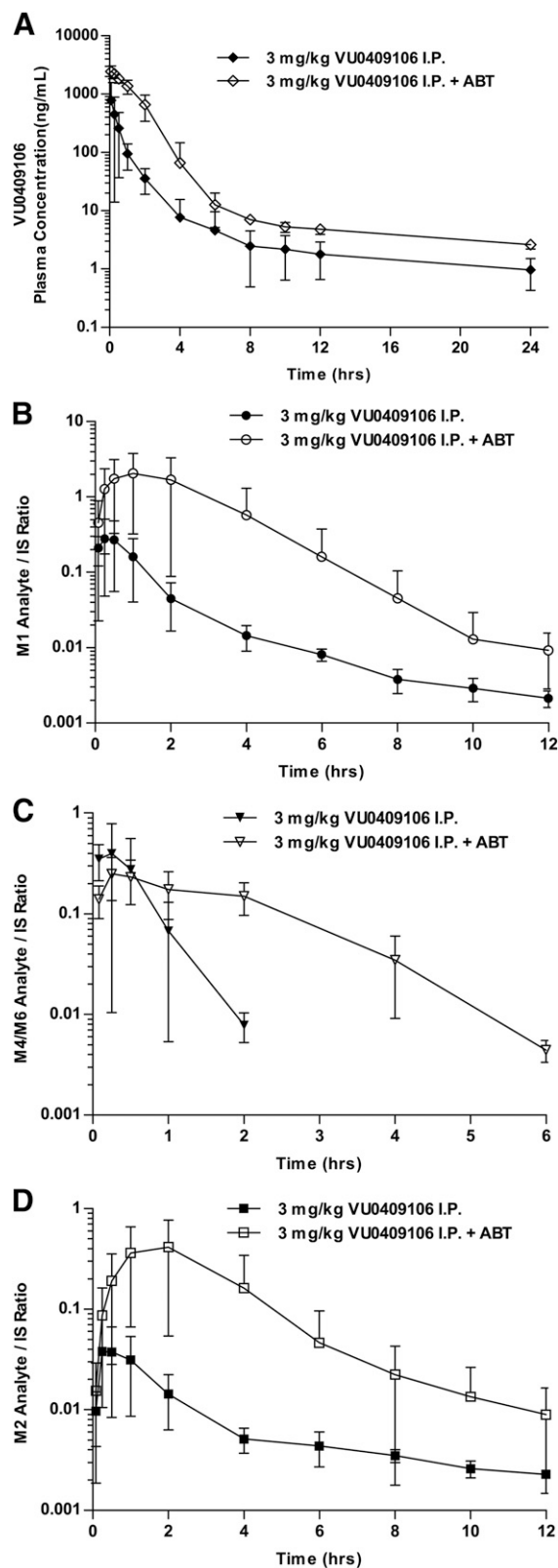
Fig. 2. Mean plasma concentration-time profiles of VU0409106 ( 1 ) (A), M1 (B), M4–M6 (C), and M2 (D) after administration of 1 to control (closed symbol) or ABT pretreated (open symbol) SD rats. Each data point represents the mean ( \pm S.D.; n = 2 or 3 (control), n = 3 or 4 ABT pretreated).
