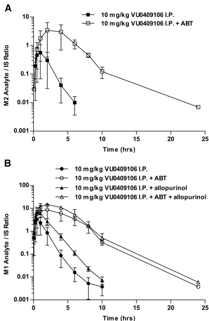
Fig. 3. Mean plasma concentration-time profiles of M2 (A) or M1 (B) after i.p. administration of VU0409106 ( 1 ) (10 mg/kg) to rats with or without an inhibitor. (A) Relative levels of M2 in rats pretreated with ABT (open squares) versus vehicle (closed squares). (B) Relative levels of M1 in rats pretreated with ABT (open circles), allopurinol (closed triangles), ABT + allopurinol (open triangles), or vehicle (closed circles). Data are expressed as the peak area ratio of analyte/internal standard and represent the mean ( \pm S.E.M., n = 2 ).
