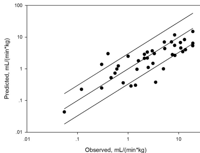
Fig. 2. The comparison of predicted vs. observed systemic CL in humans based on the optimized model in pigs. Lines shown are the line of identity and the ranges from 3-fold to 0.33-fold. Data compiled in Table A1 (Supplemental Material). Reproduced with permission of the copyright owner (Saguaro Technical Press).
