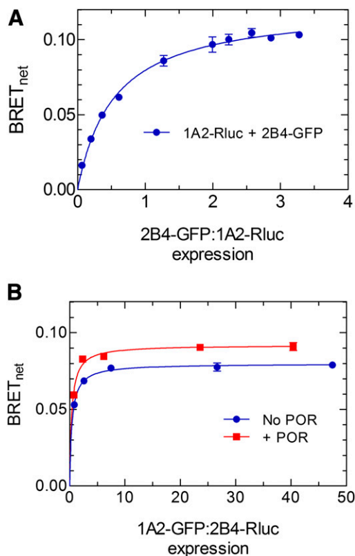
Fig. 1. Detection of physical complexes between CYP1A2 and CYP2B4 using BRET. (A) Physical complex formation between CYP2B4 and CYP1A2. pGFP 2 -N1/CYP2B4-GFP and pRluc-N2/CYP1A2-Rluc were transfected into HEK-293T/17 cells at different ratios and BRET was measured. (B) Effect of POR on the CYP1A2/CYP2B4 BRET pair. pGFP 2 -N1/CYP1A2-GFP and pRluc-N2/CYP2B4-Rluc were cotransfected into HEK-293T/17 cells (blue). This was repeated in the presence of cotransfected unlabeled POR, which did not measurably affect BRET_{max} (red), indicating that the CYP1A2-CYP2B4 complex is stable in the presence of POR. The mean \pm S.D. value for triplicate determinations is represented unless the error bars are smaller than the plotted points.
