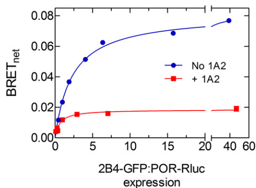
Fig. 2. Effect of unlabeled CYP1A2 on the POR/CYP2B4 BRET pair. pGFP 2 -N1/CYP2B4-GFP and pRluc-N1/POR-Rluc were cotransfected into HEK-293T/17 cells at varying GFP:Rluc ratios both in the absence (blue) and presence (red) of cotransfected, unlabeled CYP1A2. Each point represents the mean of triplicate determinations with the S.D. value within the data point.
