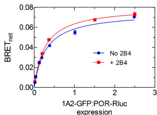
Fig. 3. Effect of unlabeled CYP2B4 on the BRET-sensitive POR-CYP1A2 complex. pGFP 2 -N1/CYP1A2-GFP and pRluc-N1/POR-Rluc were cotransfected into HEK-293T/17 cells at varying GFP:Rluc ratios in the absence (blue) and presence (red) of cotransfected unlabeled CYP2B4. Points represent the mean \pm S.D. values for three measurements; for most points, the error is smaller than the data point.
