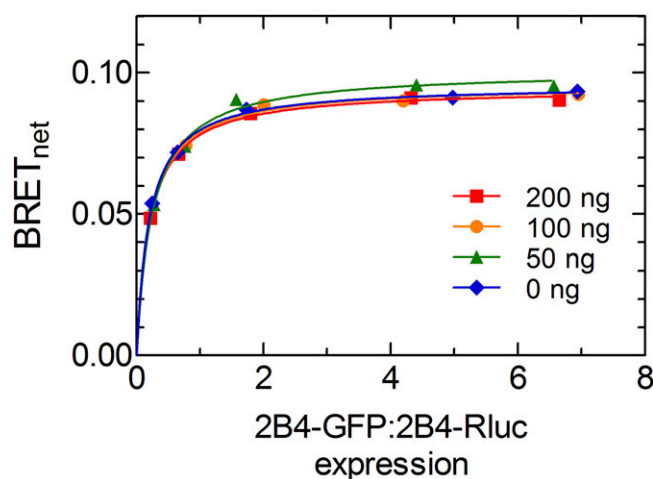
Fig. 6. Effect of unlabeled CYP2B4 on the BRET signal for the CYP2B4-CYP2B4 BRET pair. pGFP 2 -N1/CYP2B4-GFP and pRluc-N2/CYP2B4-Rluc were cotransfected into HEK-293T/17 cells, and BRET was measured in the presence and absence of different amounts of cotransfected unlabeled CYP2B4. The presence of unlabeled competitor did not have an effect on the BRET max , suggesting that CYP2B4-GFP and CYP2B4-Rluc do not form a specific BRET-detectable complex. Each point represents the mean value of triplicate determinations with the S.D. value within the data points.
