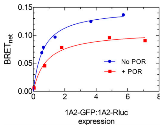
Fig. 5. Effect of unlabeled POR on the BRET signal for the CYP1A2-CYP1A2 complex. pGFP 2 -N1/CYP1A2-GFP and pRluc-N2/CYP1A2-Rluc were cotransfected into HEK-293T/17 cells, and BRET was measured (blue curve). This was repeated in the presence of cotransfected unlabeled POR (red curve). The decrease in BRET max is consistent with disruption of the CYP1A2-CYP1A2 complex. Each point represents the mean value of triplicate determinations with the S.D. value within the data points.
