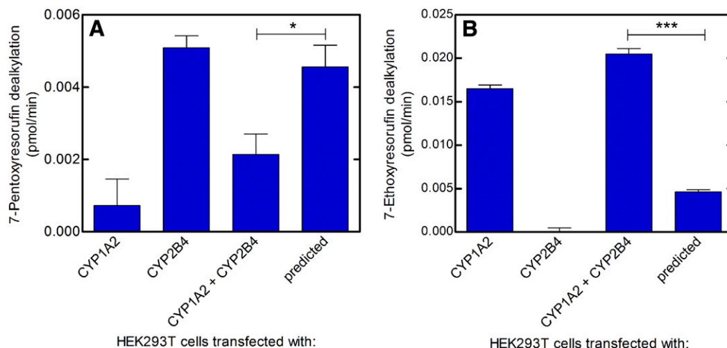
Fig. 4. Effect of cotransfection of CYP1A2-GFP and CYP2B4-GFP on PROD and EROD in microsomes isolated from transfected HEK-293T/17 cells. Cells were transfected with pGFP 2 -N1/CYP1A2-GFP, pGFP 2 -N1/CYP2B4-GFP, or both. Microsomes derived from these cells were then incubated in the presence of either 7-pentoxoresorufin or 7-ethoxoresorufin, and the initial rate of resorufin accumulation was determined spectrofluorometrically. The experimentally determined rates were then compared with those predicted for CYP1A2 and CYP2B4 if they behaved as monomers that simply competed for the available POR. Because each group of transfected cells contained different levels of POR, CYP1A2, and CYP2B4, the predicted rates were determined using Dynafit 4, based on the model described in Supplemental Fig. 1. Consequently, if the P450 enzymes affected each other's function, the experimental data would be expected to deviate from the "predicted" activities. This analysis showed that cotransfection of both P450s led to lower rates of PROD activity (A) and higher rates of EROD activity (B) than predicted by simple competition. Protein concentrations from the CYP1A2 group were 0.048 and 0.005 \mu M for CYP1A2 and POR, respectively. Concentrations for the CYP2B4 group were 0.040 and 0.005 \mu M for CYP2B4 and POR, respectively. Concentrations for the group cotransfected with both CYP1A2 and CYP2B4 were 0.051, 0.045, and 0.005 \mu M for CYP1A2, CYP2B4, and POR, respectively. The activities represent the mean \pm S.E.M. values for four replicates. Unpaired t test: * P < 0.05; *** P < 0.001 for the difference between the measured and predicted values.
