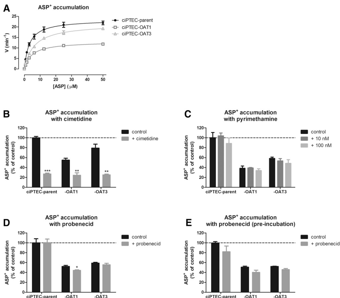
Fig. 3. Reduced ASP + accumulation reflects attenuated OCT2 transport capacity in ciPTEC-OAT1 and ciPTEC-OAT3. (A) ASP + (0.8–50 \mu M) accumulation for 60 minutes is decreased in ciPTEC-OAT1 and ciPTEC-OAT3 compared with ciPTEC-parent, evaluated by intracellular fluorescence intensity after 60 minutes (mean \pm S.E.M., n = 3 ). (B–D) ASP + (3.1 \mu M) accumulation for 60 minutes in ciPTEC-parent, ciPTEC-OAT1, and ciPTEC-OAT3 is reduced by (B) competitive inhibition of OCT (cimetidine, 1.25 mM) but not affected by competitive inhibition of (C) MATE (pyrimethamine, 10 and 100 nM) or (D) OAT (probenecid, 100 \mu M), evaluated by intracellular fluorescence intensity. Results are normalized to unexposed ciPTEC-parent (mean \pm S.E.M., n = 3 , * P < 0.05 ; ** P < 0.01 ; *** P < 0.001 ; compared with control by Student's t test). (E) ASP + (3.1 \mu M) accumulation for 60 minutes in ciPTEC-parent, ciPTEC-OAT1, and ciPTEC-OAT3 is not affected by 7-day competitive OAT inhibition (probenecid, 100 \mu M), evaluated by intracellular fluorescence intensity. Results are normalized to unexposed ciPTEC-parent (mean \pm S.E.M., n = 2 , no significant differences were found for treatment by Student's t test).
