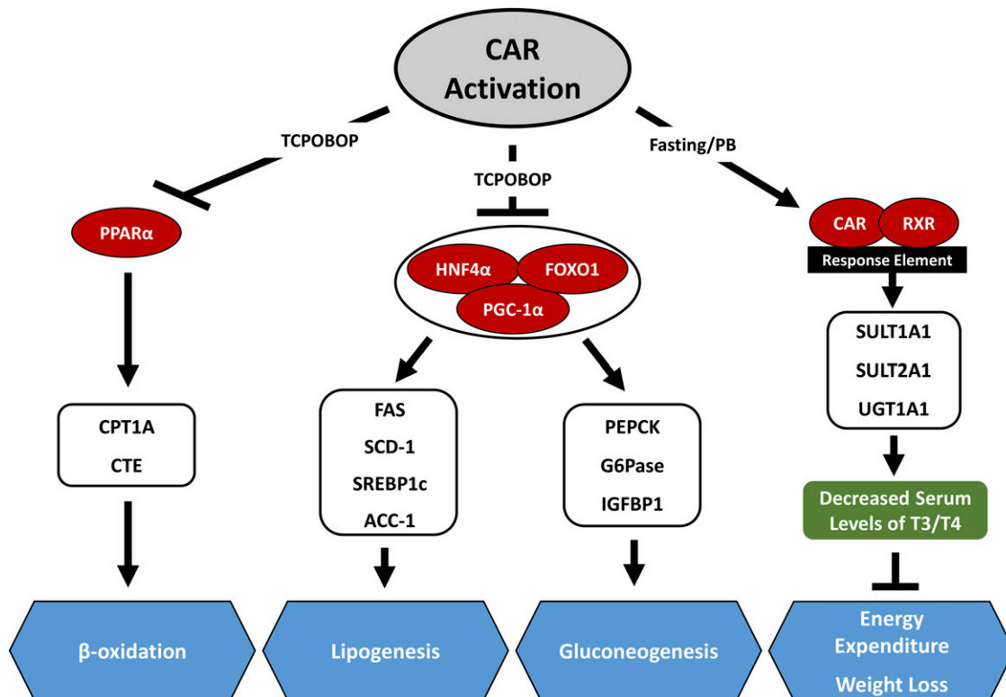
Fig. 1. Effects of CAR activation on energy homeostasis. Schematic illustration of how CAR activation affects energy metabolism and balance. Activation of CAR by agonists or caloric restriction leads to the up- and downregulation of a cluster of genes associated with gluconeogenesis, lipogenesis, \beta -oxidation, and energy expenditure by altering the activities of specific transcription factors such as peroxisome proliferator-activated receptor \alpha (PPAR \alpha ), hepatic nuclear factor-4 \alpha (HNF4 \alpha ), FOXO1, and PGC1 \alpha .
