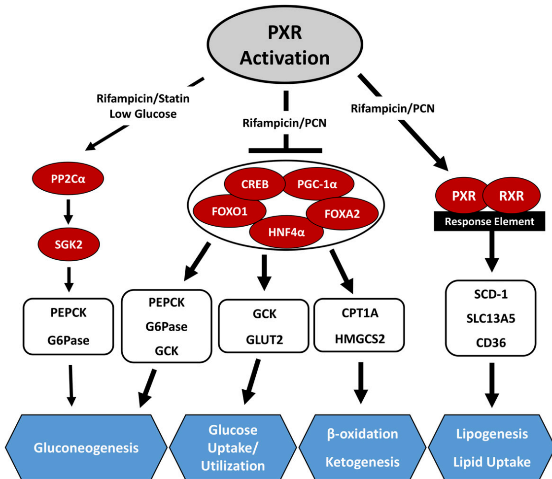
Fig. 2. Effects of PXR activation on energy homeostasis. Schematic illustration of how PXR activation affects energy metabolism and balance. Activation of PXR by agonists or low glucose results in up- and downregulation of a cluster of genes associated with gluconeogenesis, lipogenesis, and \beta -oxidation by altering the activities of specific transcription factors such as hepatic nuclear factor-4 \alpha (HNF4 \alpha ), FOXO1, FOXA2, PGC1 \alpha , and CREB, or protein phosphatases/kinases such as protein phosphatase 2C \alpha (PP2C \alpha ), and SGK2.
