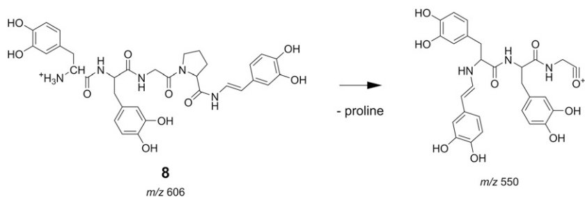
Scheme 3. Examples of gas-phase rearrangements taken from the literature (part 2).
