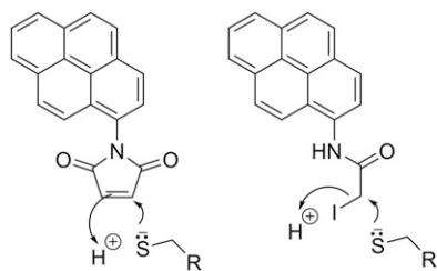
Fig. 1. Structures of PM and PIA. PM (left) and PIA (right) differ by the electrophilic group attached to a pyrene core. Arrows indicate the flow of electrons from an attacking cysteine thiolate anion nucleophile.
