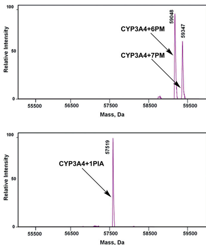
Fig. 3. Alkylation of CYP3A4 apo-protein by PM and PIA. Purified recombinant CYP3A4 (0.5 \mu M) was reacted with PIA or PM (5 \mu M) in separate tubes for 10 minutes. The samples were analyzed by high-resolution mass spectrometry, and resultant deconvoluted spectra are shown in the chromatogram for PM (top panel) and PIA (bottom panel).
