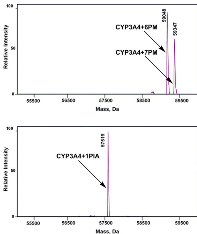
Fig. 3. Alkylation of CYP3A4 apo-protein by PM and PIA. Purified recombinant CYP3A4 (0.5 \mu M) was reacted with PIA or PM (5 \mu M) in separate tubes for 10 minutes. The samples were analyzed by high-resolution mass spectrometry, and resultant deconvoluted spectra are shown in the chromatogram for PM (top panel) and PIA (bottom panel).
