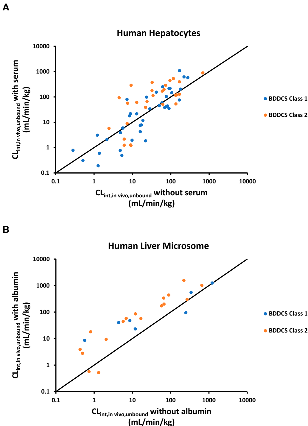
Fig. 3. Comparison of unbound intrinsic clearance from (A) hepatocyte (B) microsomal incubations with and without serum/albumin addition for BDDCS class 1 drugs (blue dots) and class 2 drugs (orange dots). Solid line is line of identity.
