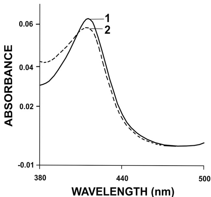
Fig. 2. Irreversible Type I spectral shift produced by the binding of 17 \alpha -ethynyl progesterone metabolite(s) to purified bovine adrenal CYP21A2 (Stevens et al., 1991). The figure was adapted with permission from Stevens JC, Jaw JY, Peng CT, and Halpert J, Mechanism-based inactivation of bovine adrenal cytochromes P450 C-21 and P450 17 alpha by 17 beta-substituted steroids. Biochemistry 30:3649–3658. Copyright 1991 American Chemical Society.
