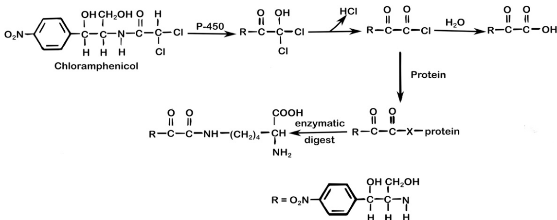
Fig. 1. Metabolic scheme for bioactivation of chloramphenicol by CYP2B1 and release of the adduct N - \epsilon -chloramphenicol oxamyl lysine upon proteolytic digestion of the modified enzyme.
