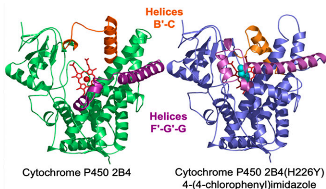
Fig. 4. Comparison of cytochrome P450 2B4 structures in the open (green) and closed, ligand-bound (blue) states, highlighting highly mobile elements of the B'C loop (orange) and F'-G helices (purple).
