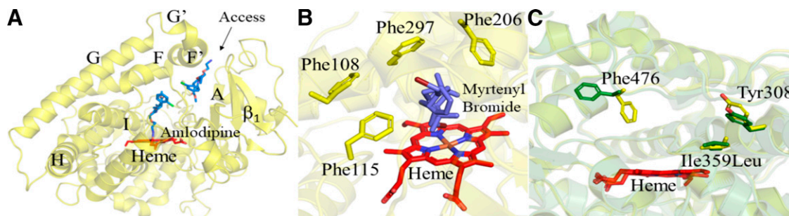
Fig. 7. Structures of human CYP2B6 and 2C9. (A) Dual ligand complex of CYP2B6 (Y226H/K262R) with amlodipine (violet sticks) bound that helped elucidate the substrate access channel from the active site near heme to the solvent region. (B) Structure of CYP2B6 (Y226H/K262R) bound with myrtenyl bromide (violet sticks) with bromine exhibiting halogen- \pi interaction with the aromatic phenylalanine side chains. (C) Structural overlay of CYP2C9 WT (green) and CYP2C9*3 (yellow) complexed with losartan. The *3 represents isoleucine to leucine change at 359 affects neighboring tyrosine at 308 that impacts the residues in the active site including phenylalanine 476. The Phe576 side chain in *3 protrudes into the active site affecting the orientation of losartan compared with the WT complex. Losartan molecules are not shown for clarity purposes. Heme is shown in red stick representation.
