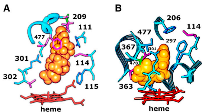
Fig. 3. Docking of ligands into the active site of the CYP2B1 model. (A) Progesterone docked into the active site of the CYP2B1 L209A mutant in a binding orientation leading to 21-OH progesterone. Key amino acid residues are shown in purple; Ala-209 is in green. Leu-209 (purple) is present in the wild type (WT) enzyme, which leads to van der Waals overlaps with progesterone. (B) BBT ( N -benzyl-1-aminobenzotriazole) docked into the active site of CYP 2B1 in an orientation allowing for oxidation at the 1-amino nitrogen, leading to enzyme inactivation. When Gly-478 is replaced with Ala, van der Waals overlaps appear between the inhibitor and the Ala side chain. Key residues are in purple, and Ala-478 is in green. Such overlaps likely account for the resistance of G478A to inactivation by the chloramphenicol analog N -(2- p -nitrophenethyl)chlorofluoroacetamide (He et al., 1992).
