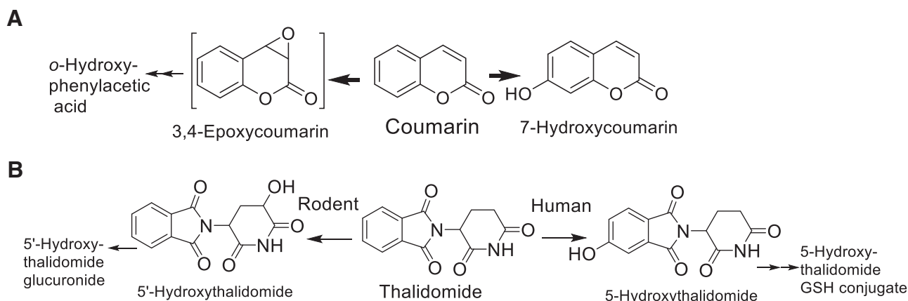
Fig. 1. Oxidation of coumarin to o -hydroxyphenylacetic acid and 7-hydroxycoumarin (A) (Miura et al., 2021a) and of thalidomide to 5'-hydroxythalidomide and 5-hydroxythalidomide (B) (Kuwagata et al., 2021; Miura et al., 2021b).
