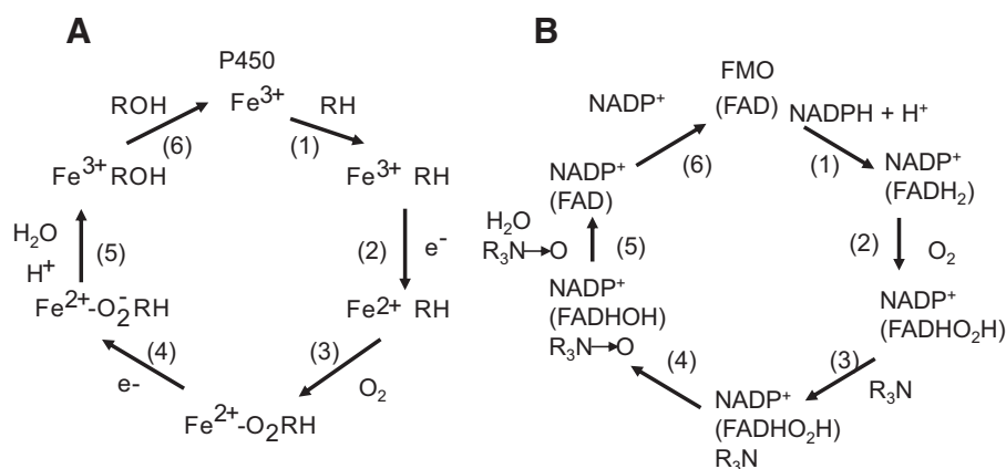
Fig. 2. Catalytic cycles of P450s (A) and FMOs (B). As indicated in the catalytic cycle, ferrous P450 can bind substrate (Yamazaki et al., 1996; Yamazaki et al., 2001), whereas for FMOs, only in the third step is the flavin hydroperoxide intermediate capable of oxygenating substrates (Ziegler, 2002).
