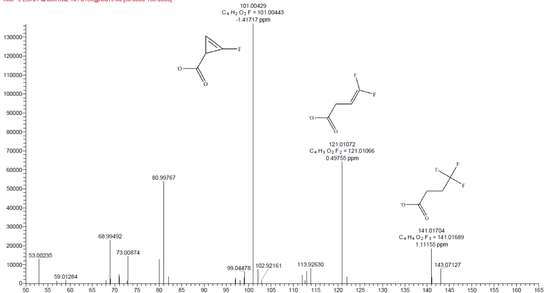
Figure S1: annotated MS/MS spectrum for metabolite M19 in fractionated human urine (fraction 19, acquired in negative-ion mode).
