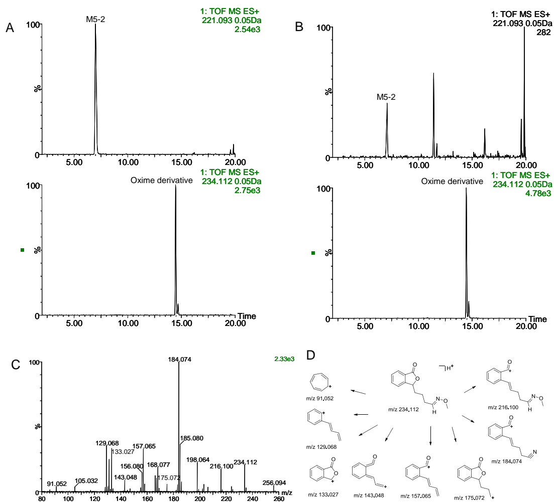
Fig. S2. Extracted ion chromatograms of m/z 221.093 (M5-2) and of m/z 234.112 (protonated ion of the potential oxime derivative) from the incubation of 11-hydroxy-NBP in human liver cytosol (A) and HLMs (B), respectively, in the presence of methoxyamine. Mass spectrum (C) and the proposed fragmentation pattern (D) of the oxime derivative.
