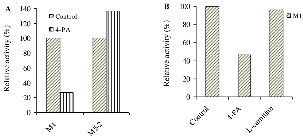
Fig. S4. Effect of 4-pentenoic acid (4-PA, 1 mM) on the formation of M5-2 and M1 from the incubation of NBP in freshly prepared rat liver homogenate (A); and the effect of 4-PA (1 mM) and L-carnitine (1 mM) on M1 production from the incubation of M5-2 in freshly prepared rat liver homogenate (B). Data are reported as the mean of two separate determinations.
