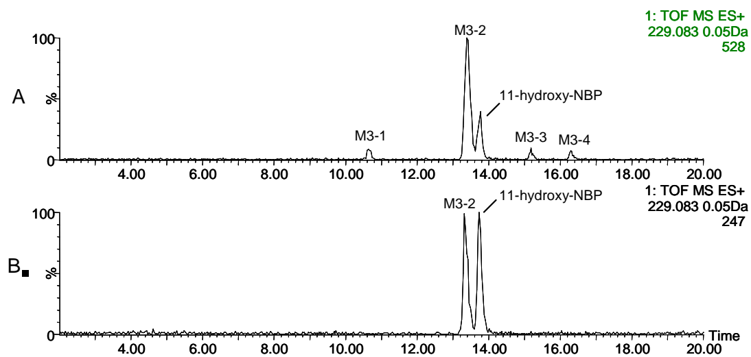
Fig. S1. Extracted ion chromatograms of m/z 229.083 (sodium adducted ion of hydroxylated NBP) from the incubation of NBP in NADPH-supplemented HLMs (A) and in the mixed solution of M3-2 and 11-hydroxy-NBP (B).
