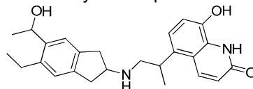
Hydroxyindacaterol
