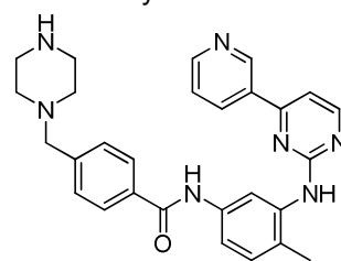
Desmethylimatinib
