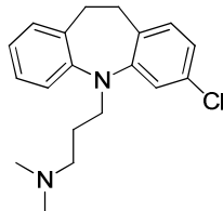
Clomipramine
