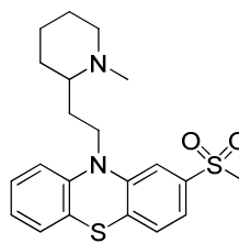
Thioridazine sulfoxide-2
