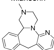
Mirtazapine
