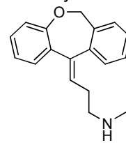
Desmethyldoxepin
