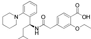
Repaglinide
