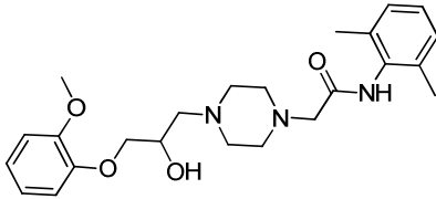
Ranolazine
