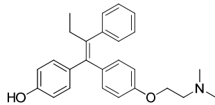
Hydroxytamoxifen
