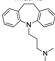
Imipramine
