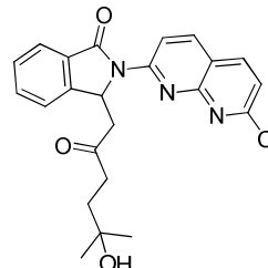
Hydroxypagoclone
