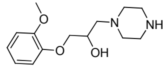
Desalkylranolazine
