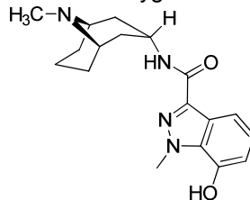
Hydroxygranisetron
