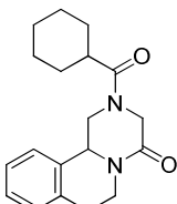
Praziquantel
