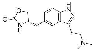
Zolmitriptan
