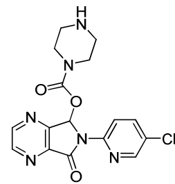
Desmethylzopiclone
