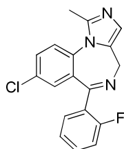
Midazolam
