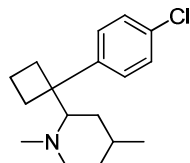
Sibutramine
