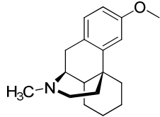
Dextromethorphan
