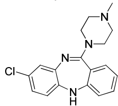
Clozapine
