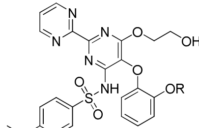
R = CH 3 , Bosentan R = H, Hydroxy metabolite
