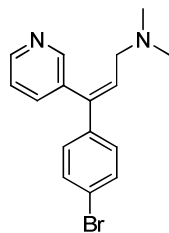
Zimelidine
