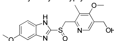
Hydroxyomeprazole
