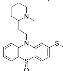
Thioridazine sulfoxide-2
