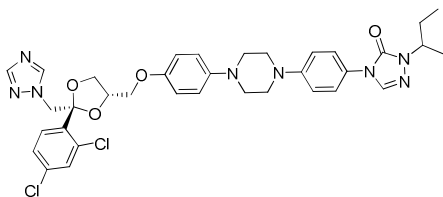
Itraconazole
