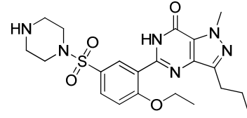
Desmethylsildenafil
