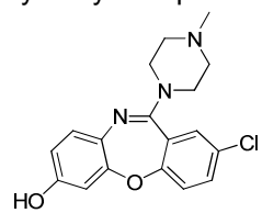
7-Hydroxyloxapine
