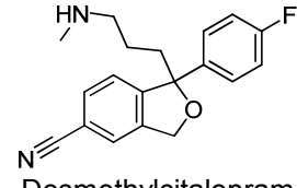
Desmethylcitalopram
