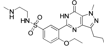
Cleaved piperazine ring
