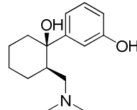
Demethoxytramadol
