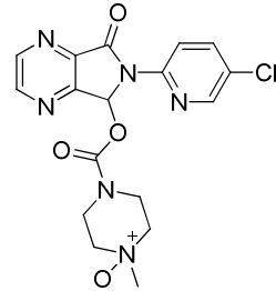
Zopiclone N-oxide
