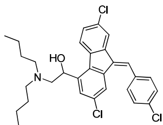
Lumefantrine
