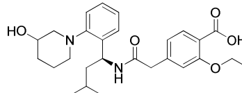
Hydroxyrepaglinide
