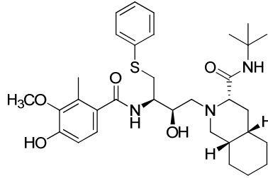
Methoxycathecol
