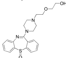
Quetiapine sulfoxide
