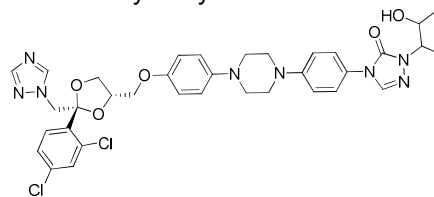
Hydroxyitraconazole
