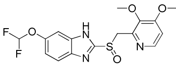
Pantoprazole
