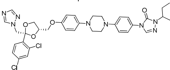
Itraconazole
