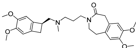
Ivabradine
