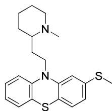
Thioridazine
