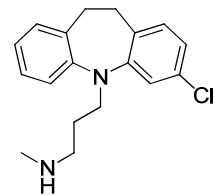
Desmethylclomipramine
