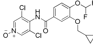
Roflumilast N-oxide
