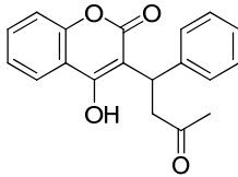
S-Warfarin
