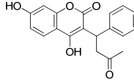
Hydroxywarfarin
