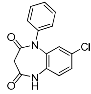
Norclobazam
