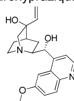
Hydroxyquinidine
