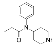
Norfentanyl
