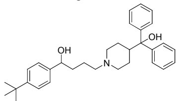
Terfenadine
