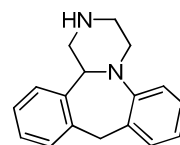
Desmethylmianserin
