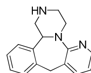
Desmethylmirtazapine
