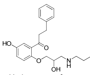
Hydroxypropafenone
