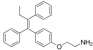
Didesmethyltamoxifen
