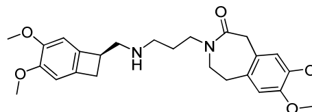
Desmethylivabradine
