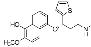
5-Hydroxy-6-methoxy duloxetine
