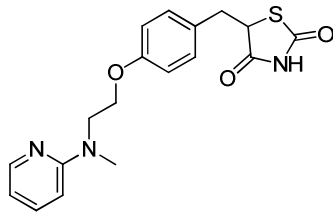
Rosiglitazone
