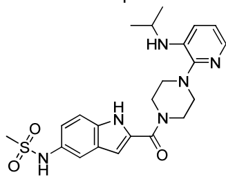
Delavirdine
