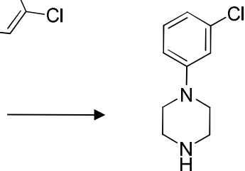
m-Chlorophenylpiperazine cLogD = 0.56
