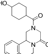
Hydroxypraziquantel
