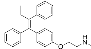
Desmethyltamoxifen
