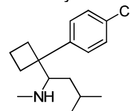
Desmethylsibutramine
