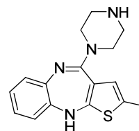
Desmethylolanzapine
