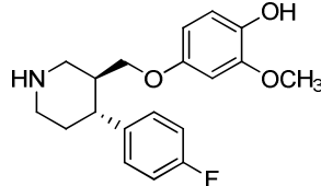
4-Hydroxy-3-Methoxy Paroxetine
