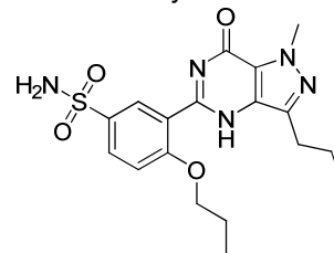
Desalkyludenafil
