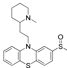
Thioridazine sulfoxide (Mesoridazine)
