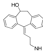
Hydroxynortryptiline
