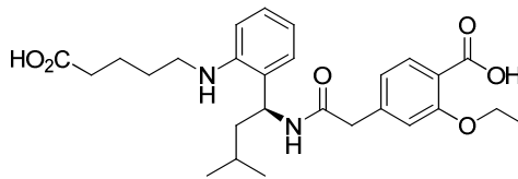
Carboxylic Acid Metabolite
