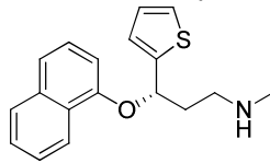
Duloxetine
