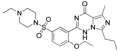
Vardenafil
