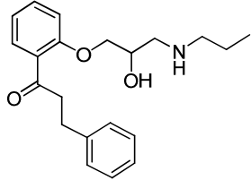
Propafenone
