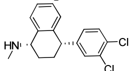
Sertraline
