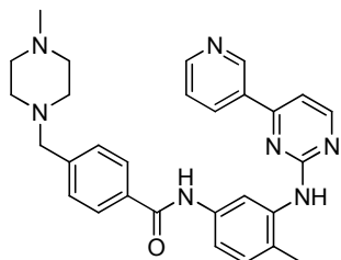
Imatinib
