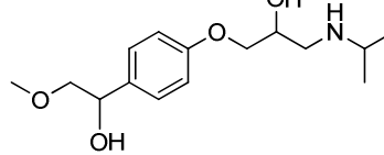
\alpha -Hydroxymetoprolol
