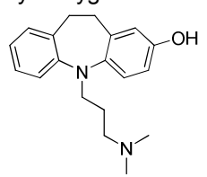
Hydroxyimipramine
