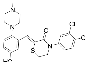
5-HydroxyElzasonan
