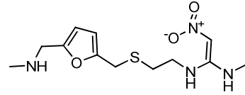
Desmethylranitidine
