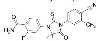
Desmethylenzalutamide
