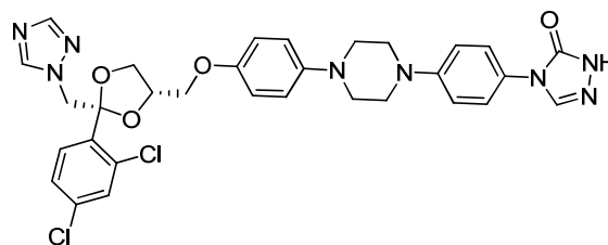
Dealkylitraconazole
