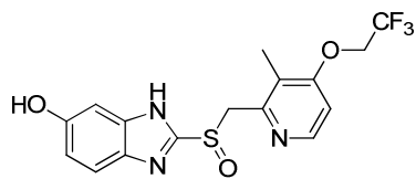
Hydroxylansoprazole
