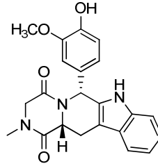
4-Hydroxy-3-Methoxy Tadalafil
