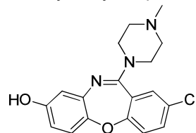
8-Hydroxyloxapine
