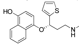
Hydroxyduloxetine
