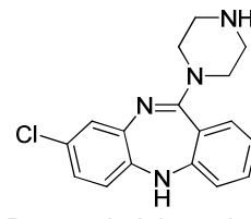
Desmethylclozapine
