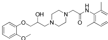
Ranolazine
