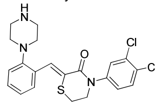
Desmethyl elzasonan
