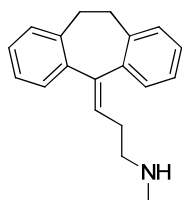
Nortryptiline
