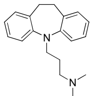
Imipramine
