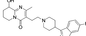
Hydroxyrisperidone
