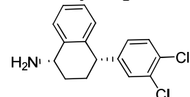
Desmethylsertraline
