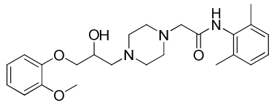
Ranolazine
