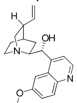
Quinidine
