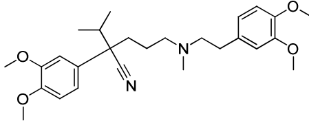
Verapamil
