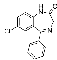
Desmethyldiazepam
