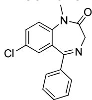
Diazepam
