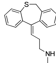
Desmethyldothiepin
