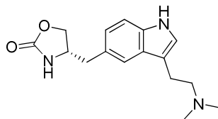
Zolmitriptan
