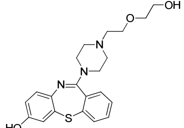
Hydroxyquetiapine
