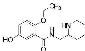
Dealkyloxyflecainide
