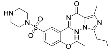
Desethylvardenafil
