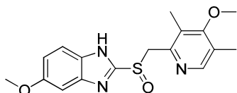
Omeprazole
