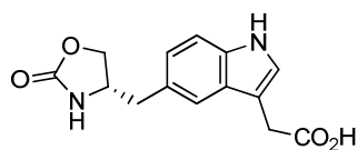
Zolmitriptan indoleacetic acid
