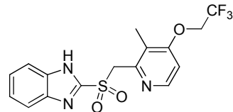
Lansoprazole sulfone
