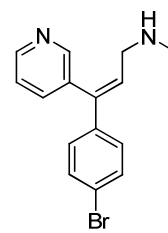
Desmethylzimelidine
