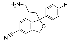
Didesmethylcitalopram
