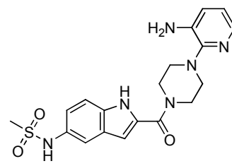
Desisopropyl delavirdine
