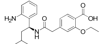
Dealkylregaplinide (M1)
