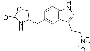
Zolmitriptan N-oxide
