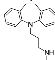
Desipramine
