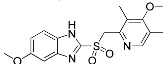
Omeprazole sulfone
