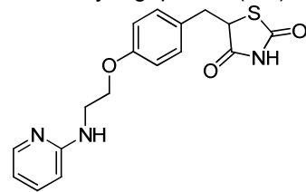
Desmethylrosiglitazone
