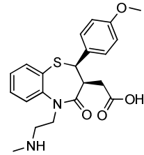
Desmethyldiltiazem
