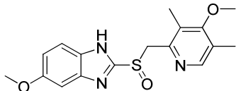
Omeprazole
