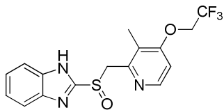
Lansoprazole
