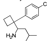
Didesmethylsibutramine
