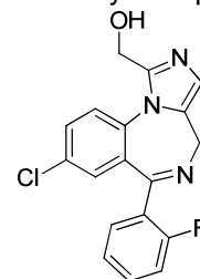
1'-Hydroxymidazolam
