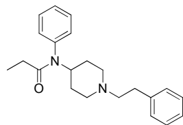
Fentanyl
