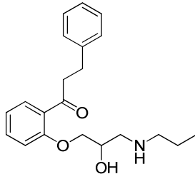
Propafenone
