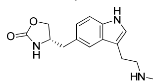
Desmethylzolmitriptan
