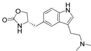
Zolmitriptan
