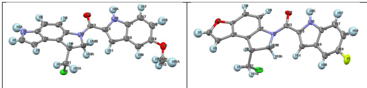
Figure S1. Structures of ( R )-ICT2700 and ( R )-ICT2726 as determined by single molecule X-ray crystallography. Thermal ellipsoids drawn at 50% probability level.
